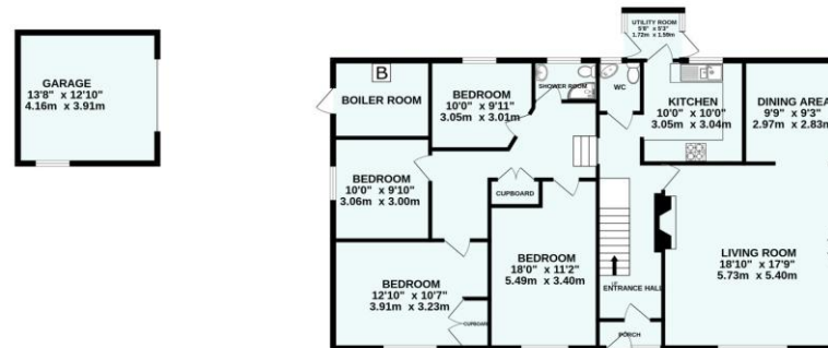
1ST FLOOR 769 sq.ft. (71.4 sq.m.) approx.
