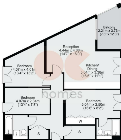
Fourth Floor
