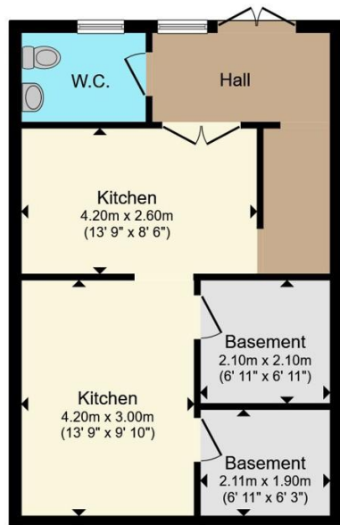
Basement
