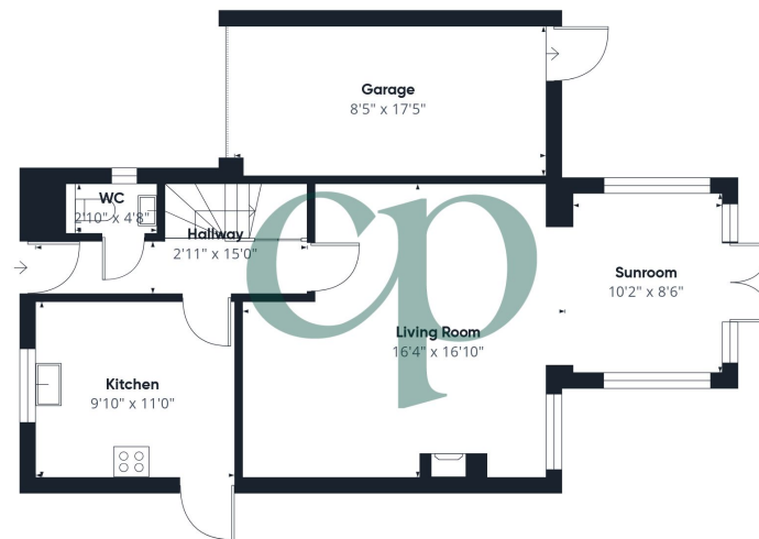
Floor 0
