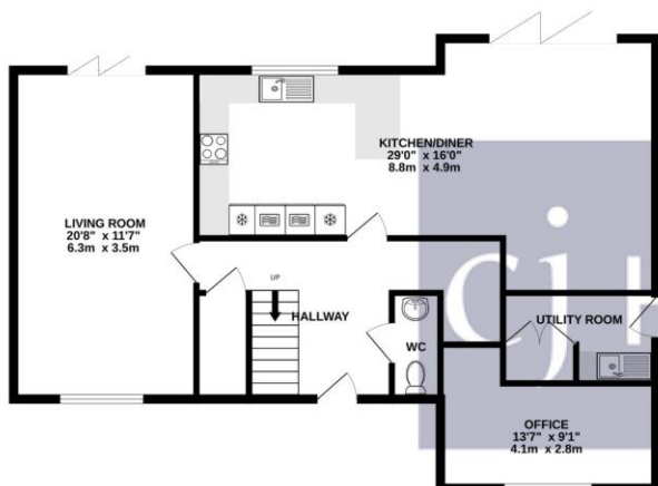
GROUND FLOOR 942 sq.ft. (87.5 sq.m.) approx.
